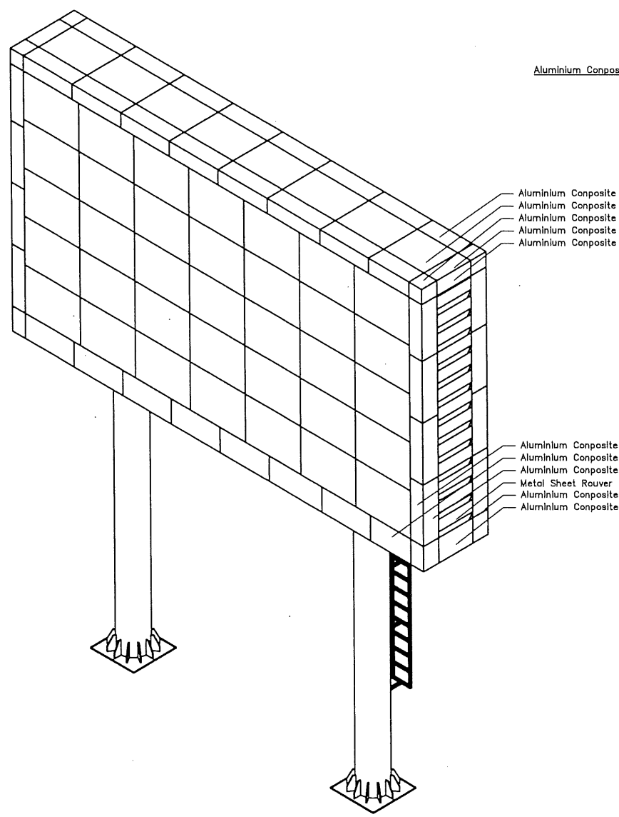
ISOMETRIC VIEW
