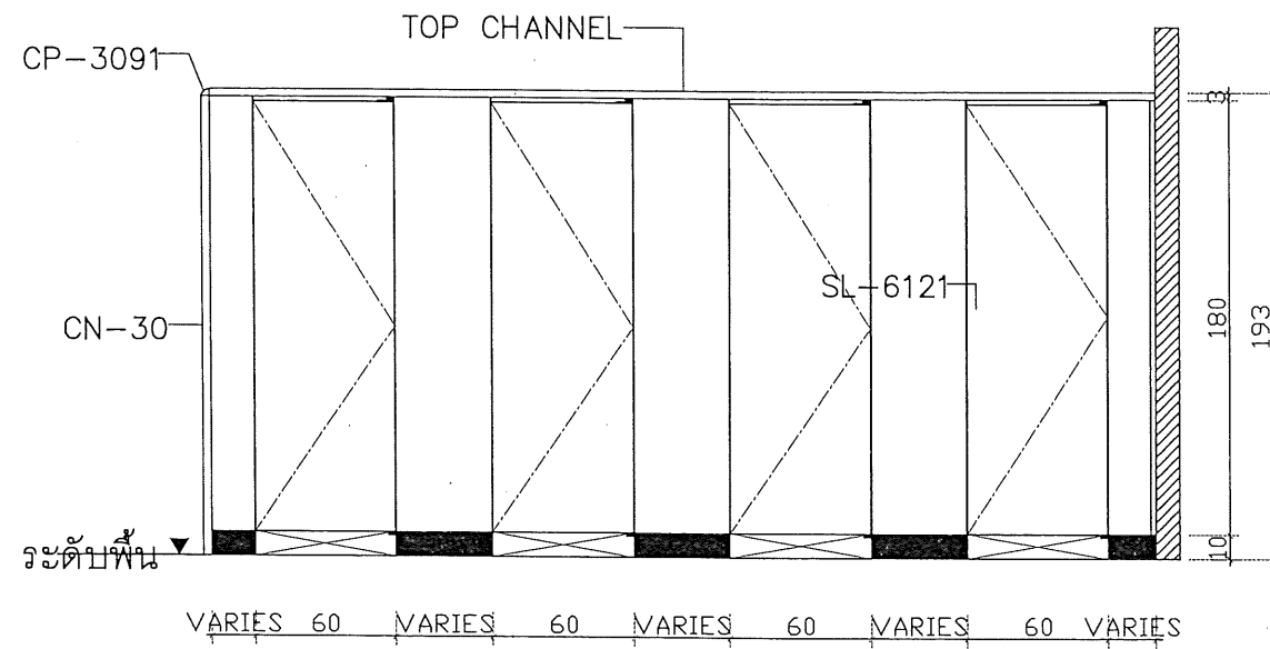
Frontview Toilet Parttion Full Door Fitting Stainless scale 1:35
