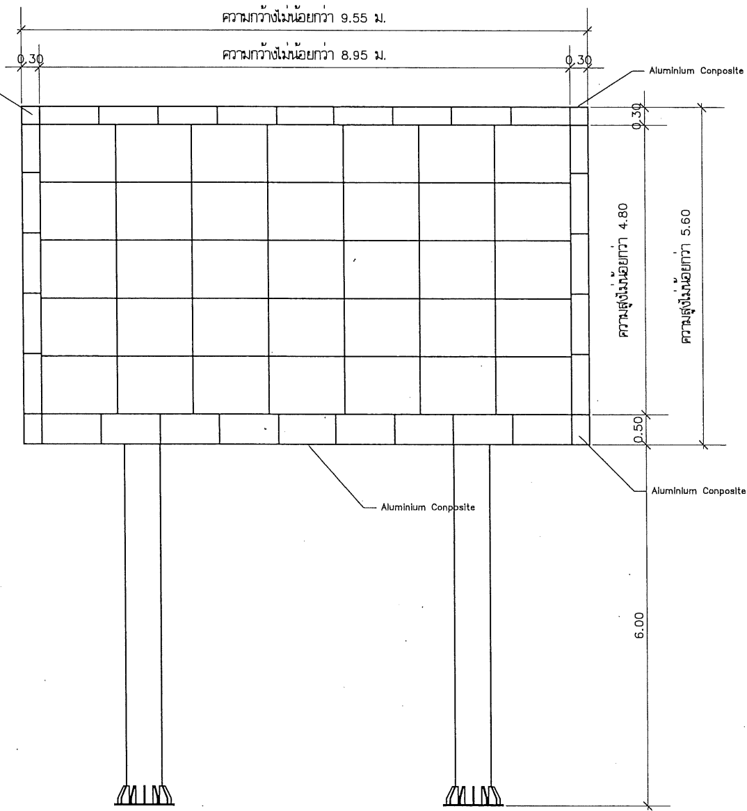
FRONT VIEW
